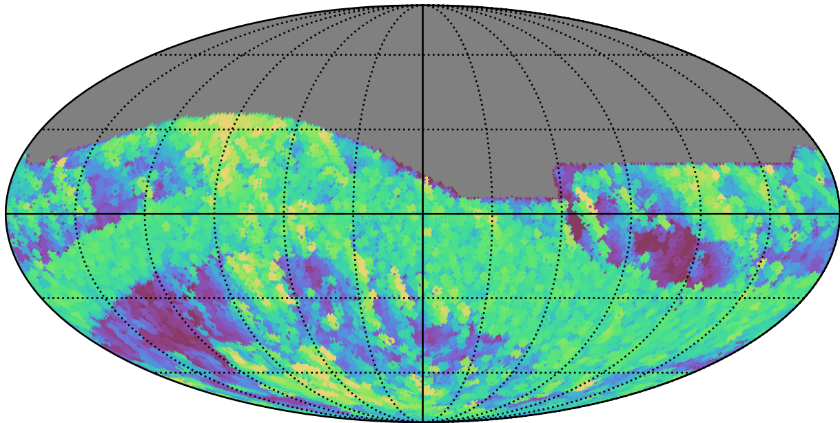
too_elab_r64_d3_giz_v3.4_10yrs All sky r band: Max airmass
