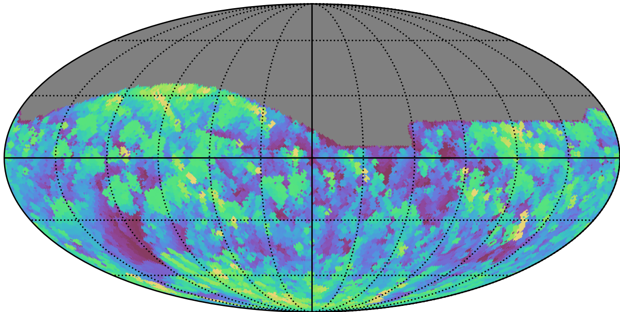
too_elab_r64_d3_giz_v3.4_10yrs All sky g band: Max airmass
