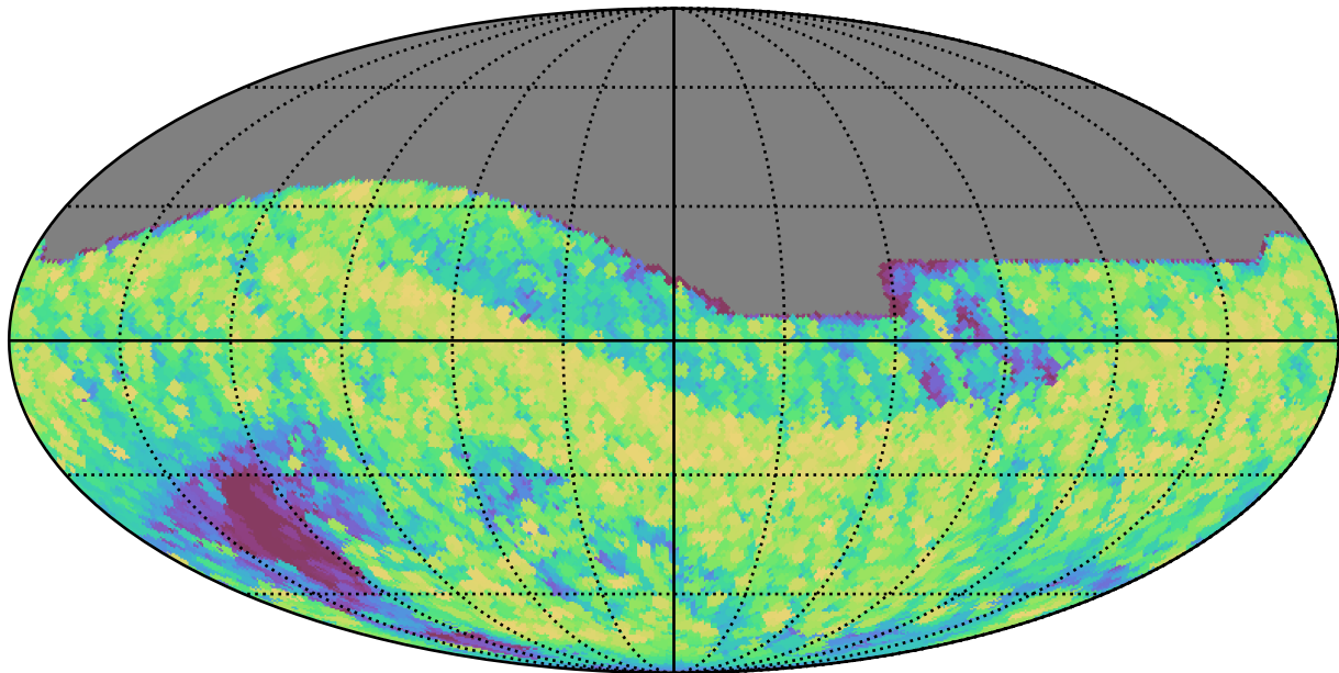
too_elab_r64_d3_giz_v3.4_10yrs All sky all bands: Max airmass
