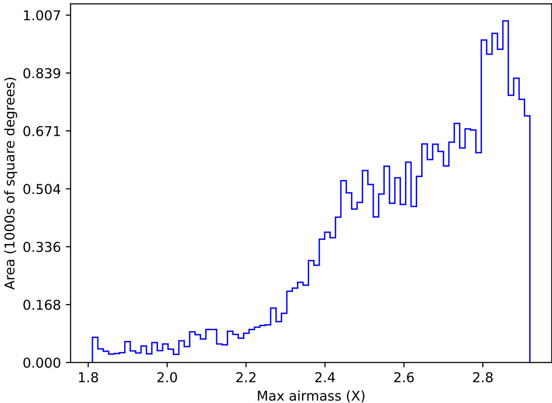
too_elab_r64_d3_giz_v3.4_10yrs All sky all bands: Max airmass
