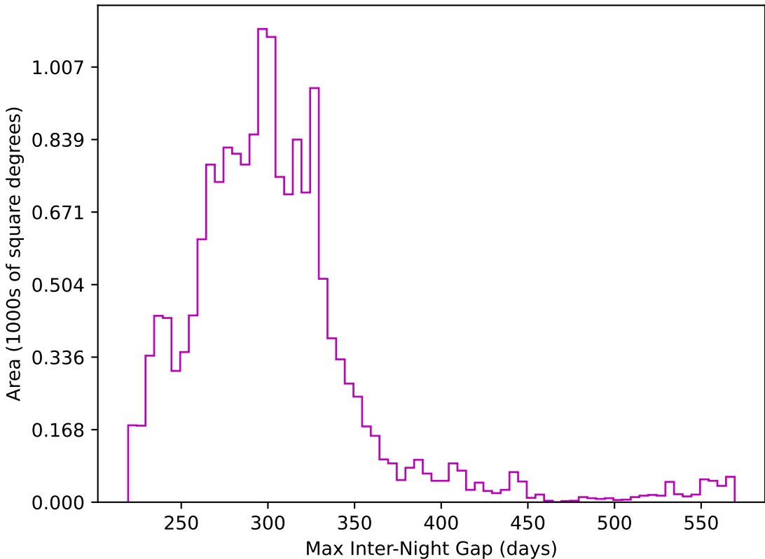
too_elab_r64_d3_giz_v3.4_10yrs WFD z band: Max Inter-Night Gap
