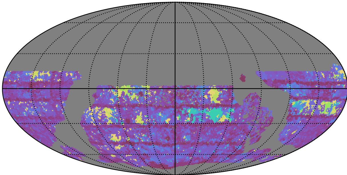
too_elab_r64_d3_giz_v3.4_10yrs WFD y band: Max Inter-Night Gap
