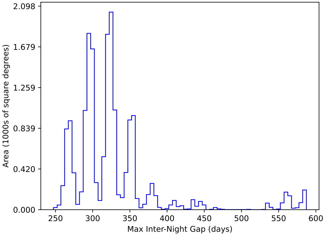
too_elab_r64_d3_giz_v3.4_10yrs WFD y band: Max Inter-Night Gap
