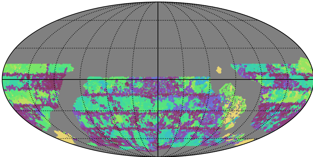
too_elab_r64_d3_giz_v3.4_10yrs WFD u band: Max Inter-Night Gap
