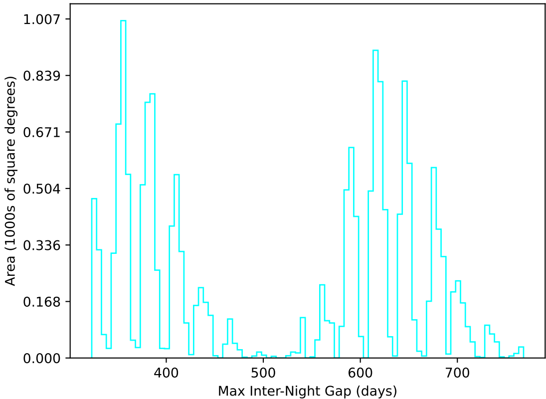
too_elab_r64_d3_giz_v3.4_10yrs WFD u band: Max Inter-Night Gap
