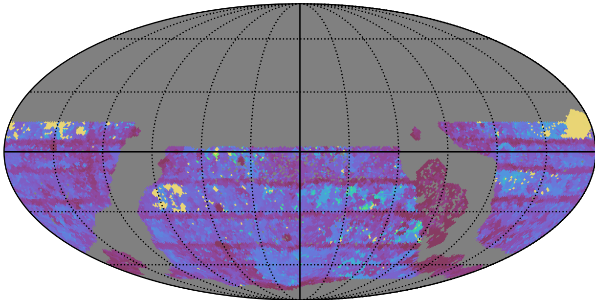
too_elab_r64_d3_giz_v3.4_10yrs WFD r band: Max Inter-Night Gap
