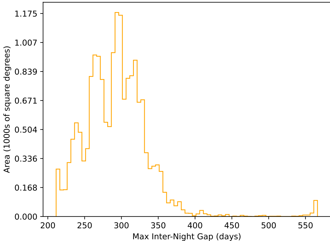
too_elab_r64_d3_giz_v3.4_10yrs WFD r band: Max Inter-Night Gap
