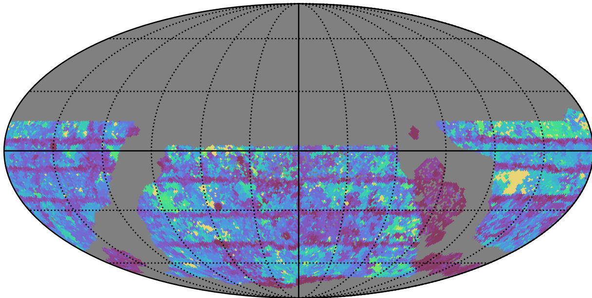
too_elab_r64_d3_giz_v3.4_10yrs WFD i band: Max Inter-Night Gap
