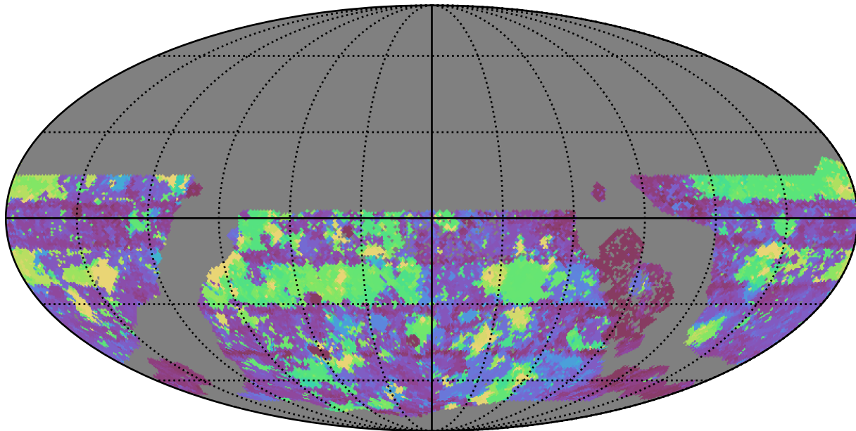
too_elab_r64_d3_giz_v3.4_10yrs WFD g band: Max Inter-Night Gap
