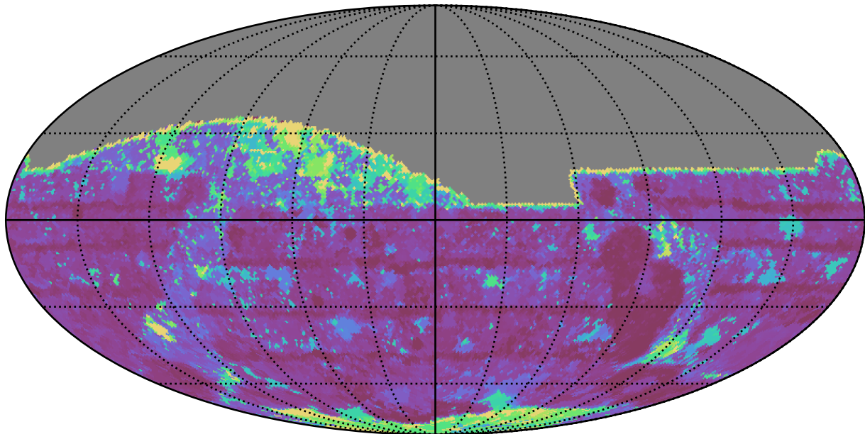
too_elab_r64_d3_giz_v3.4_10yrs All sky z band: Max Inter-Night Gap
