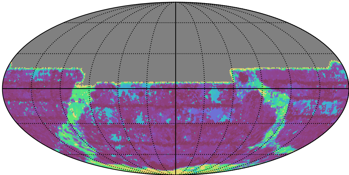
too_elab_r64_d3_giz_v3.4_10yrs All sky y band: Max Inter-Night Gap
