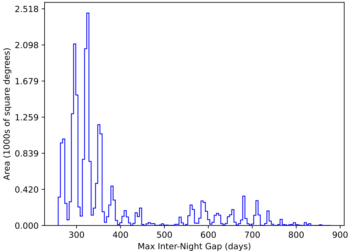
too_elab_r64_d3_giz_v3.4_10yrs All sky y band: Max Inter-Night Gap
