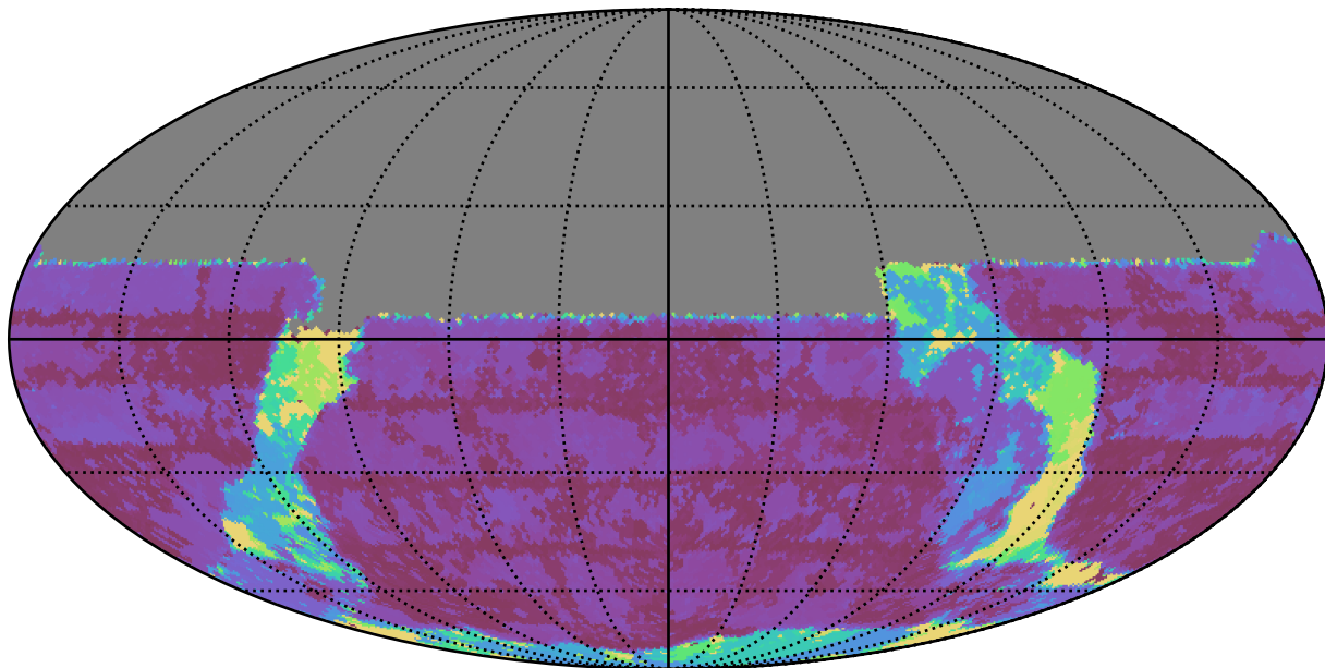
too_elab_r64_d3_giz_v3.4_10yrs All sky u band: Max Inter-Night Gap
