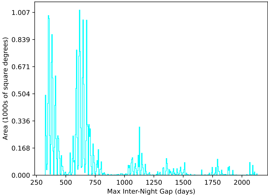
too_elab_r64_d3_giz_v3.4_10yrs All sky u band: Max Inter-Night Gap
