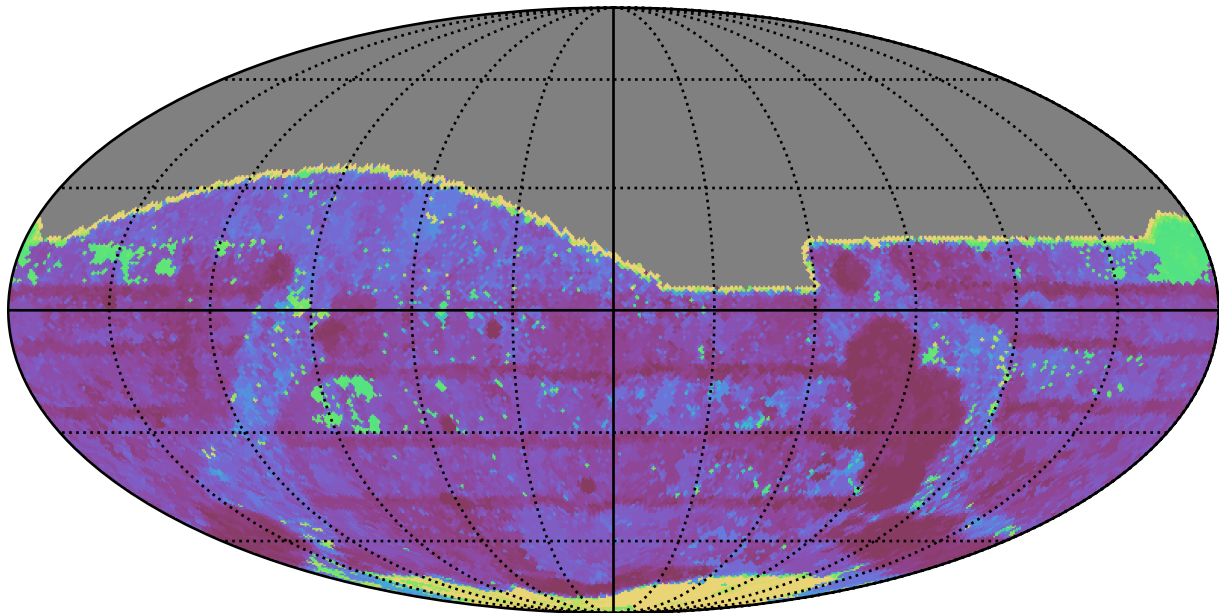
too_elab_r64_d3_giz_v3.4_10yrs All sky r band: Max Inter-Night Gap
