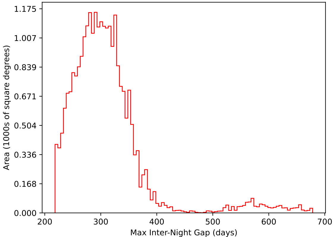
too_elab_r64_d3_giz_v3.4_10yrs All sky i band: Max Inter-Night Gap
