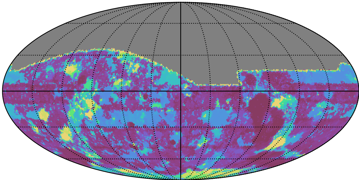
too_elab_r64_d3_giz_v3.4_10yrs All sky g band: Max Inter-Night Gap
