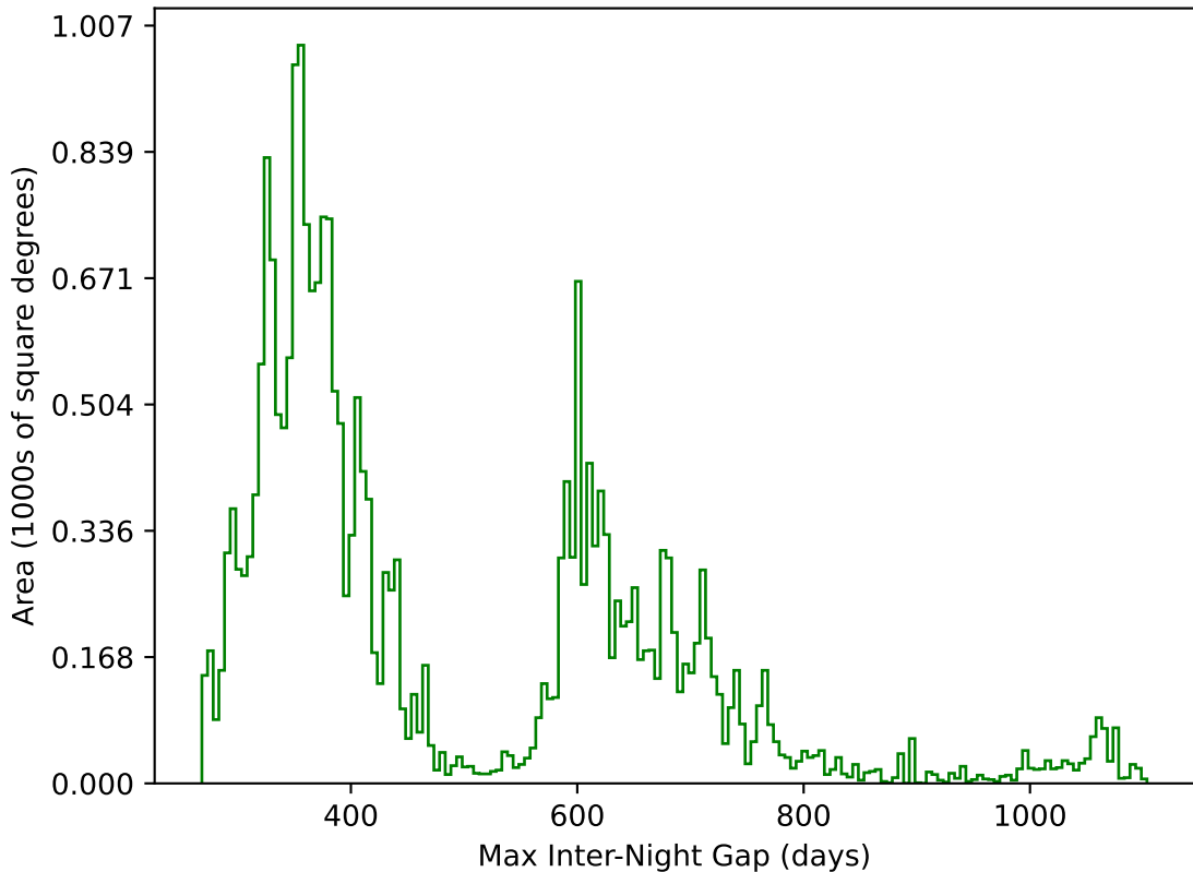
too_elab_r64_d3_giz_v3.4_10yrs All sky g band: Max Inter-Night Gap
