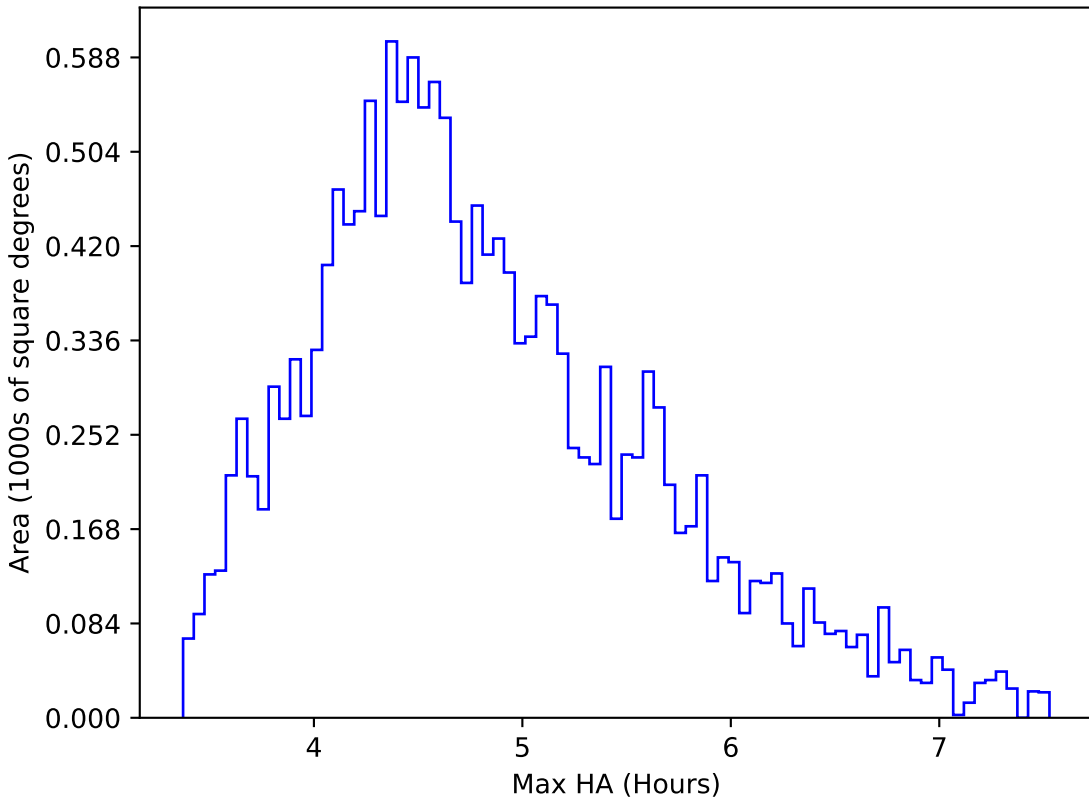
too_elab_r64_d3_giz_v3.4_10yrs WFD y band: Max HA
