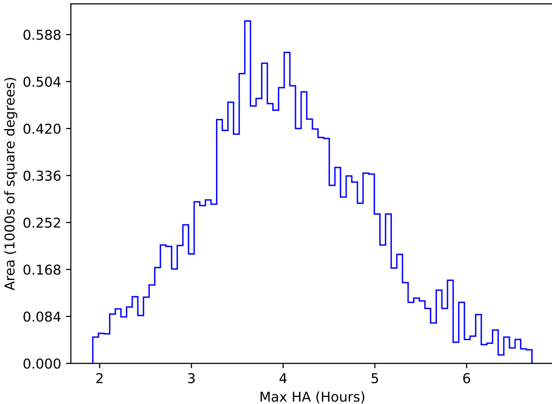
too_elab_r64_d3_giz_v3.4_10yrs WFD u band: Max HA
