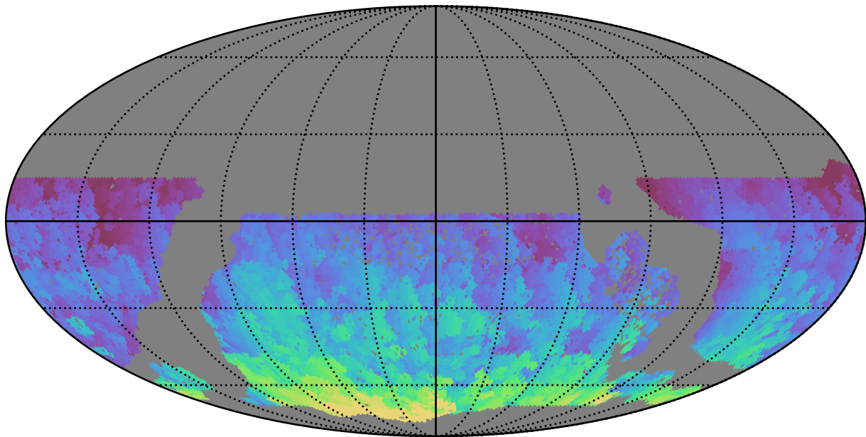
too_elab_r64_d3_giz_v3.4_10yrs WFD r band: Max HA
