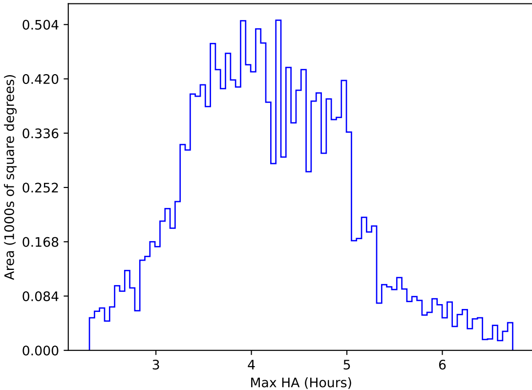
too_elab_r64_d3_giz_v3.4_10yrs WFD g band: Max HA
