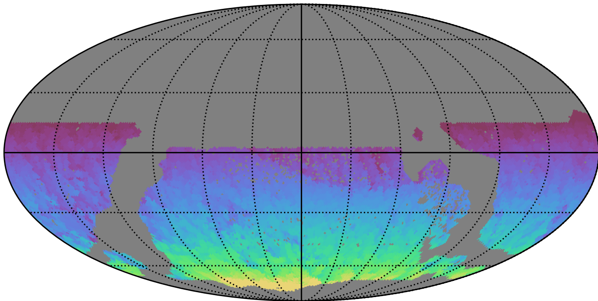
too_elab_r64_d3_giz_v3.4_10yrs WFD all bands: Max HA
