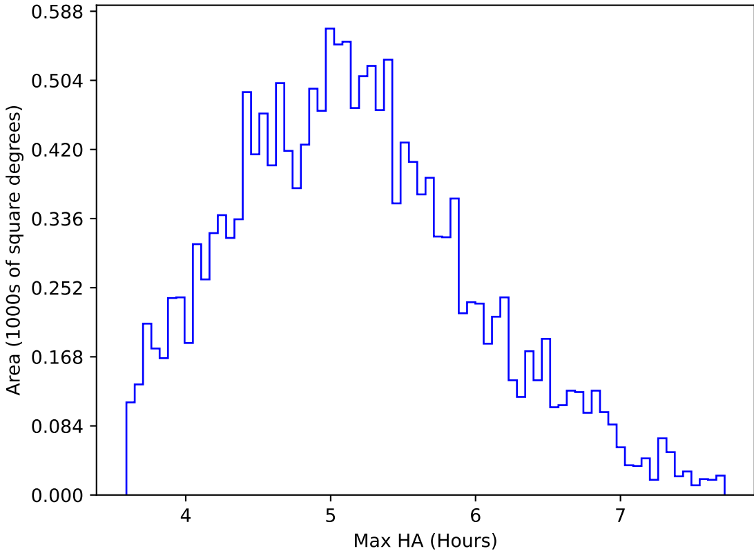
too_elab_r64_d3_giz_v3.4_10yrs WFD all bands: Max HA
