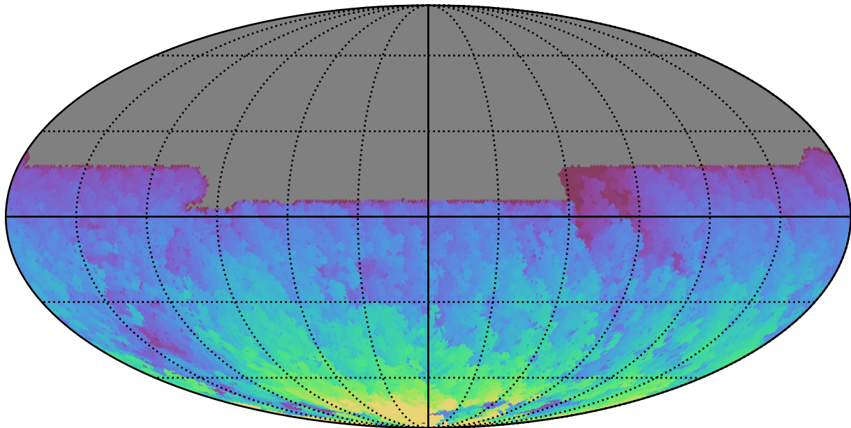
too_elab_r64_d3_giz_v3.4_10yrs All sky y band: Max HA
