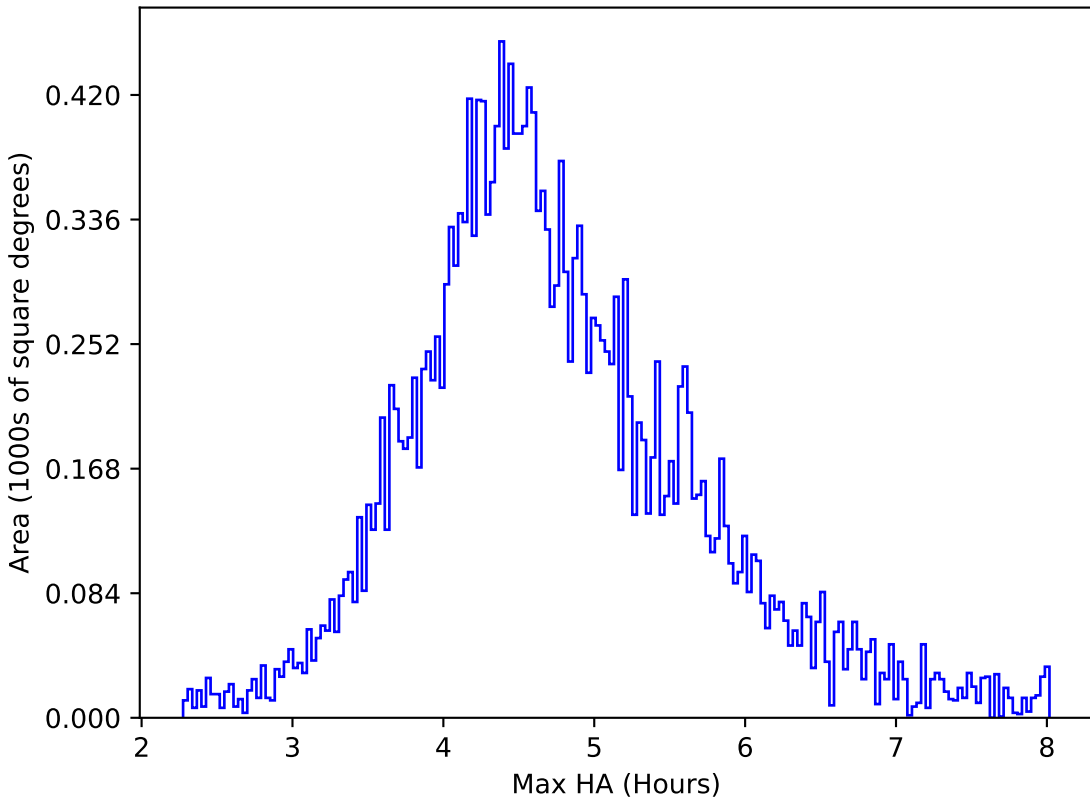
too_elab_r64_d3_giz_v3.4_10yrs All sky y band: Max HA
