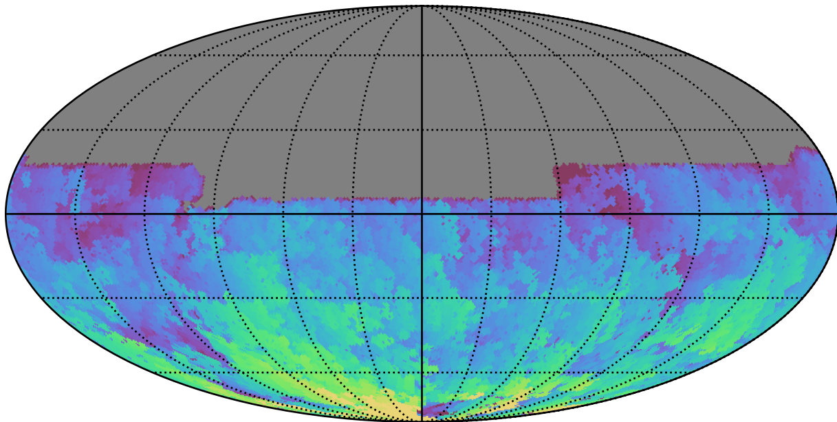
too_elab_r64_d3_giz_v3.4_10yrs All sky u band: Max HA
