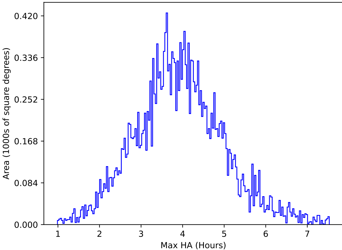
too_elab_r64_d3_giz_v3.4_10yrs All sky u band: Max HA
