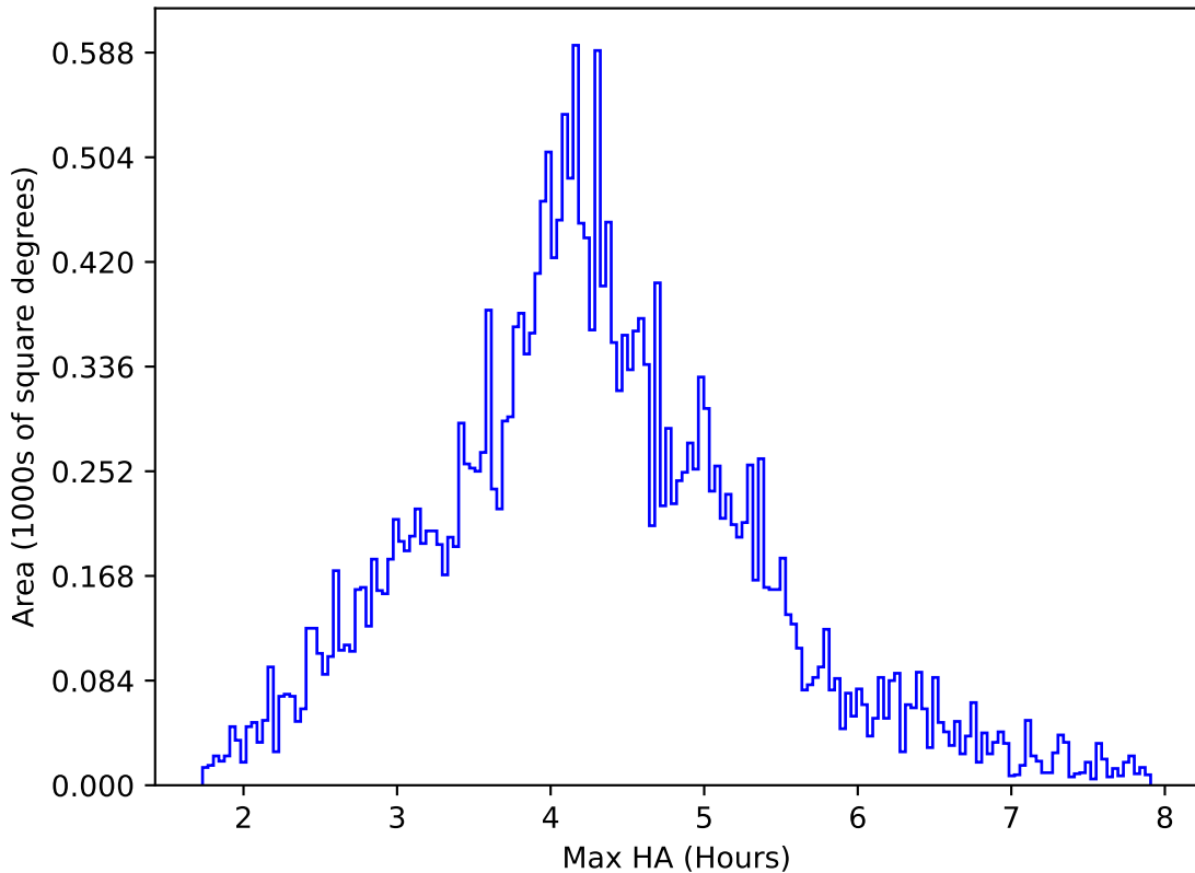
too_elab_r64_d3_giz_v3.4_10yrs All sky r band: Max HA
