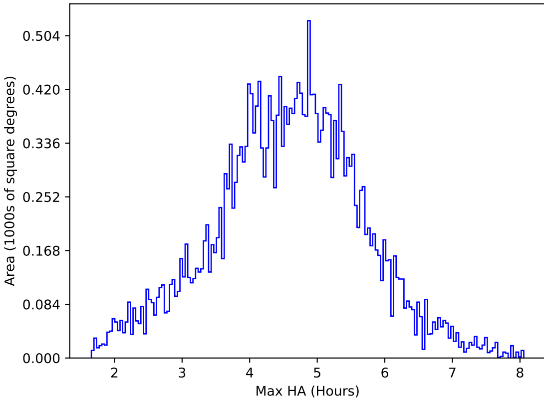
too_elab_r64_d3_giz_v3.4_10yrs All sky i band: Max HA
