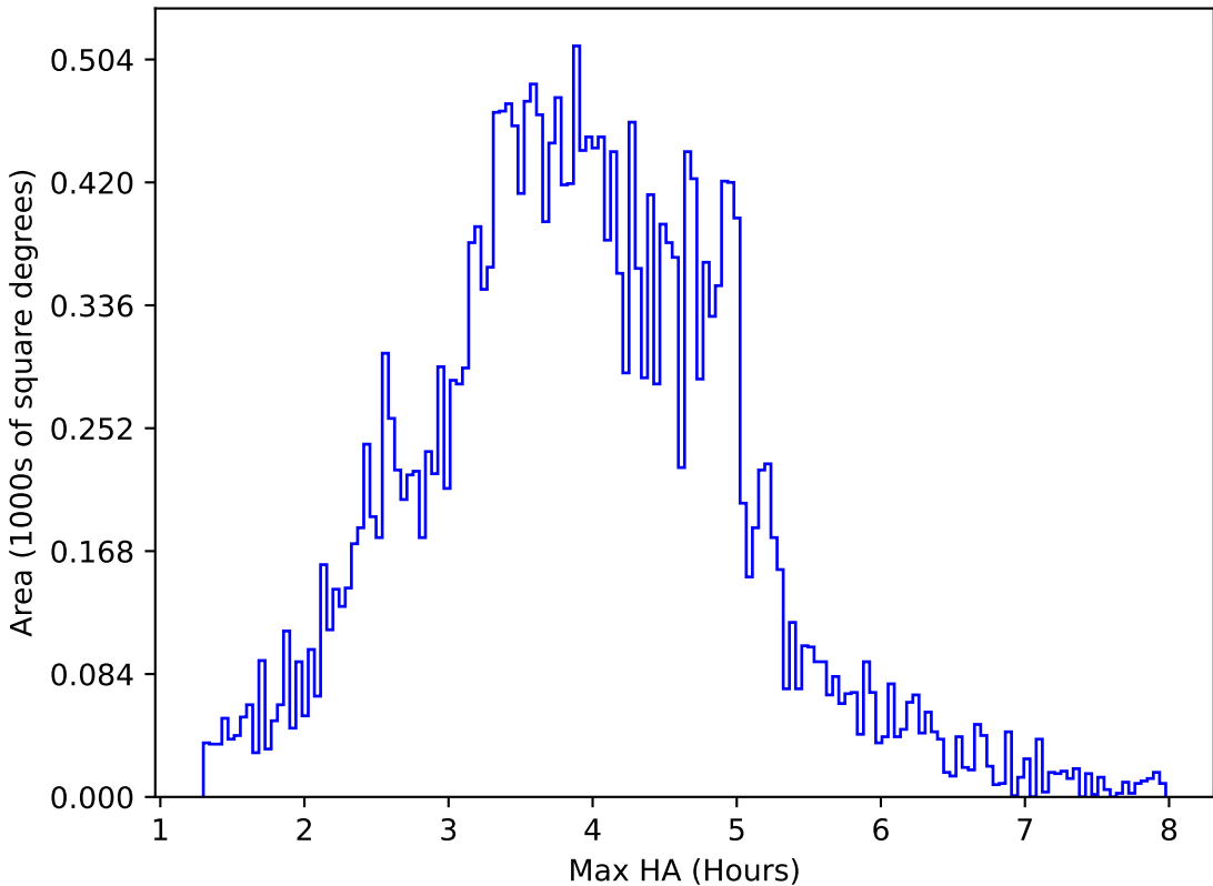
too_elab_r64_d3_giz_v3.4_10yrs All sky g band: Max HA
