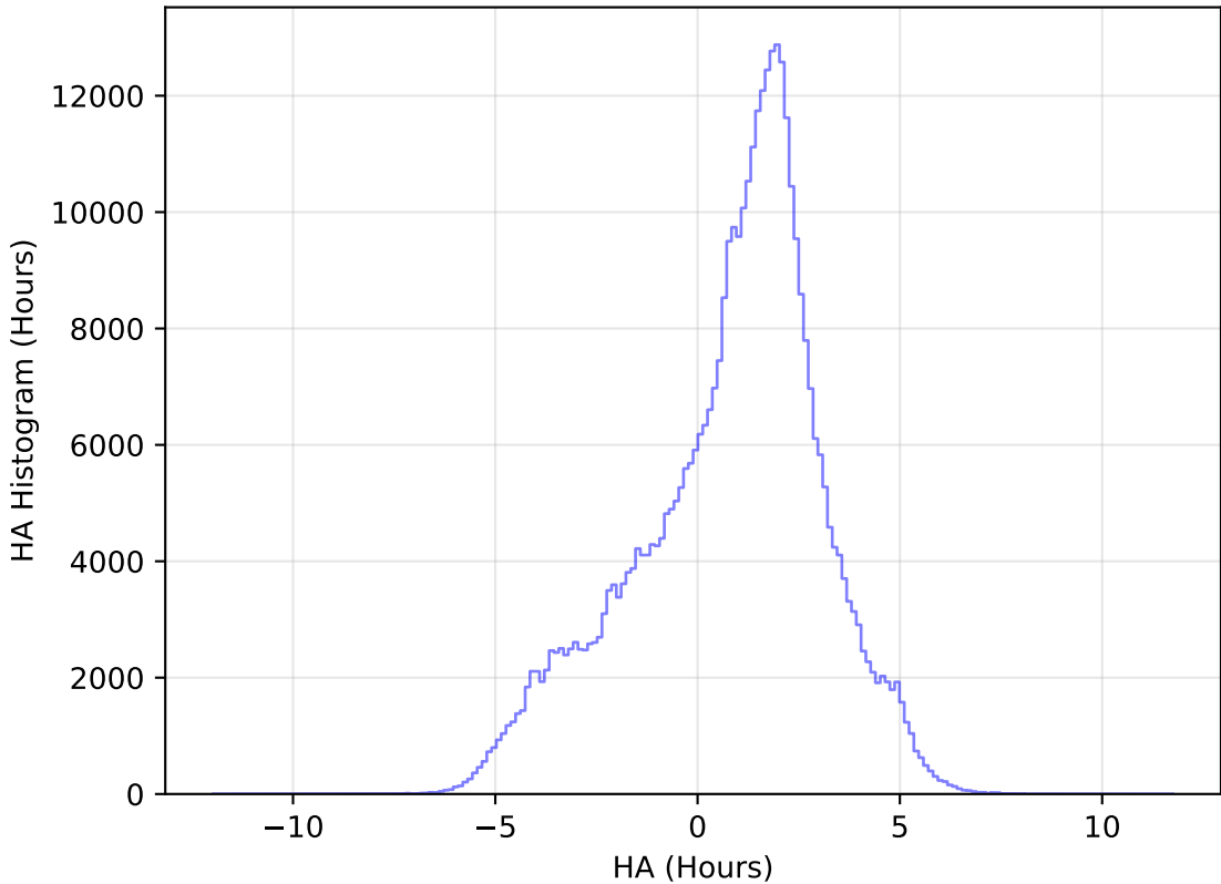
too_elab_r64_d3_giz_v3.4_10yrs WFD z band: HA Histogram
