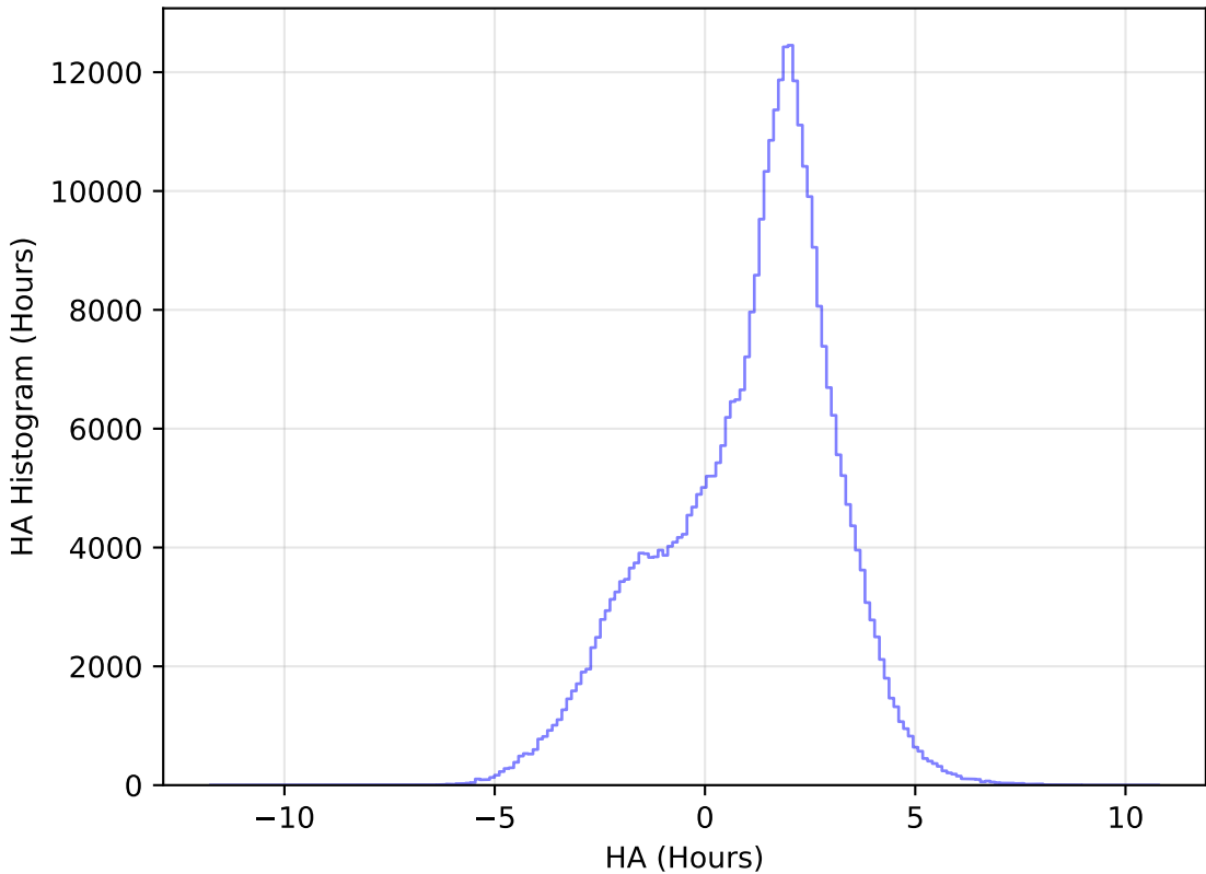
too_elab_r64_d3_giz_v3.4_10yrs WFD y band: HA Histogram
