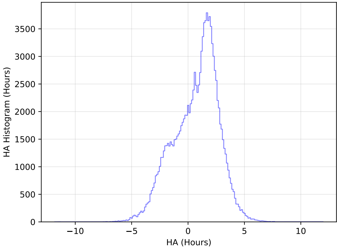
too_elab_r64_d3_giz_v3.4_10yrs WFD u band: HA Histogram
