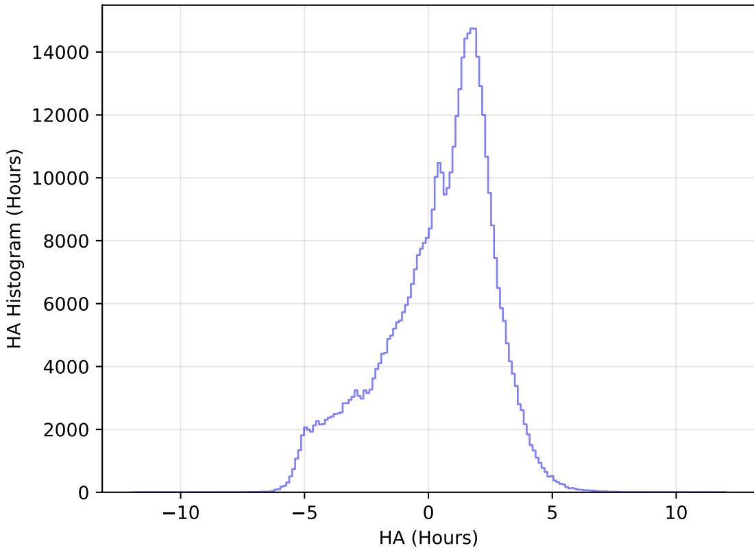
too_elab_r64_d3_giz_v3.4_10yrs WFD r band: HA Histogram
