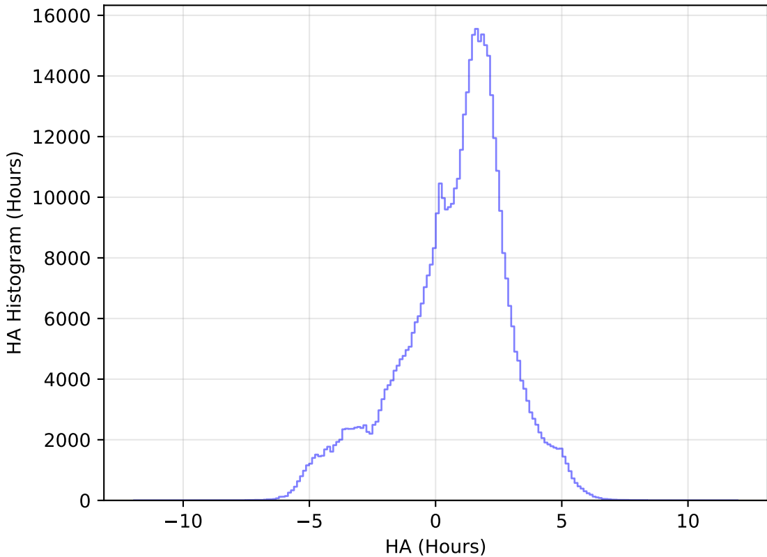
too_elab_r64_d3_giz_v3.4_10yrs WFD i band: HA Histogram
