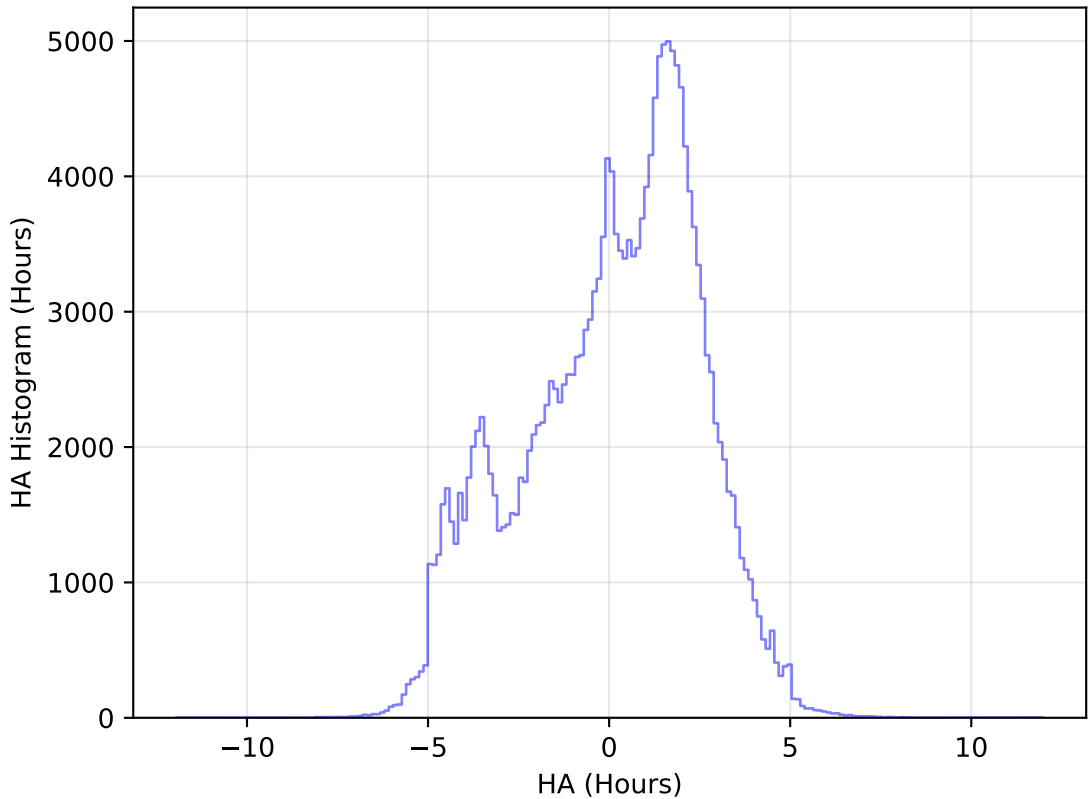
too_elab_r64_d3_giz_v3.4_10yrs WFD g band: HA Histogram
