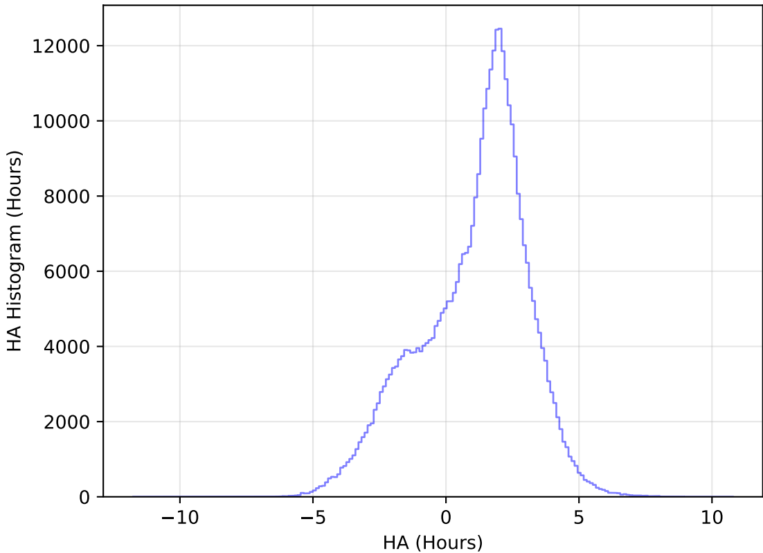
too_elab_r64_d3_giz_v3.4_10yrs All sky y band: HA Histogram
