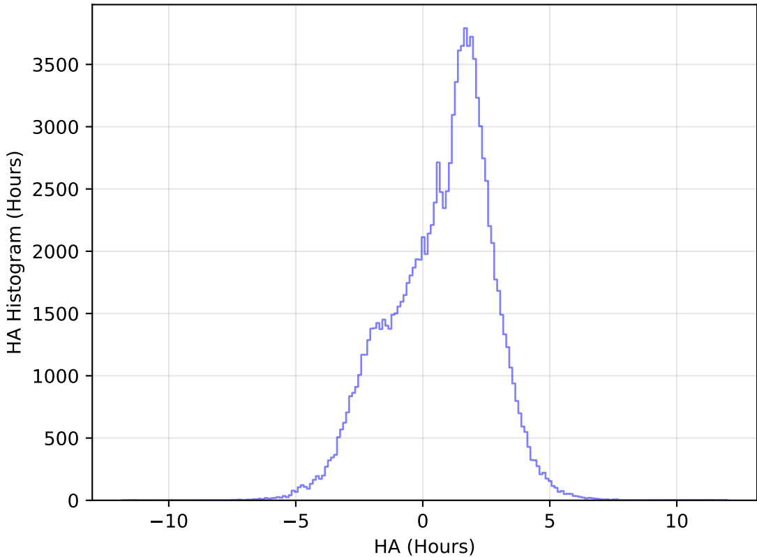
too_elab_r64_d3_giz_v3.4_10yrs All sky u band: HA Histogram
