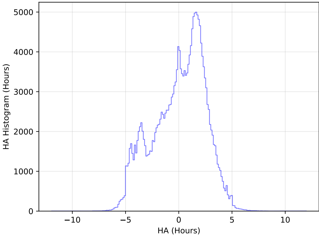
too_elab_r64_d3_giz_v3.4_10yrs All sky g band: HA Histogram
