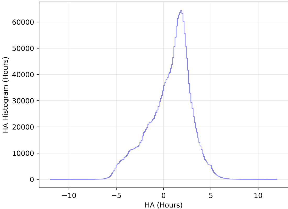
too_elab_r64_d3_giz_v3.4_10yrs All sky all bands: HA Histogram
