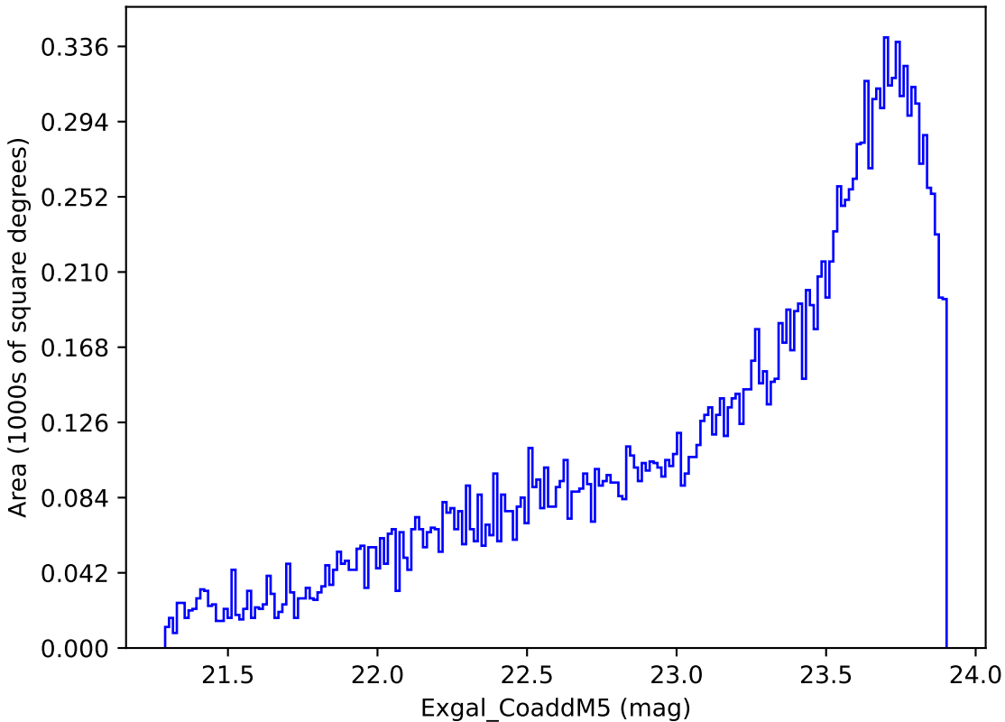
too_elab_r64_d3_giz_v3.4_10yrs Yr 3-4 y band: Exgal_CoaddM5
