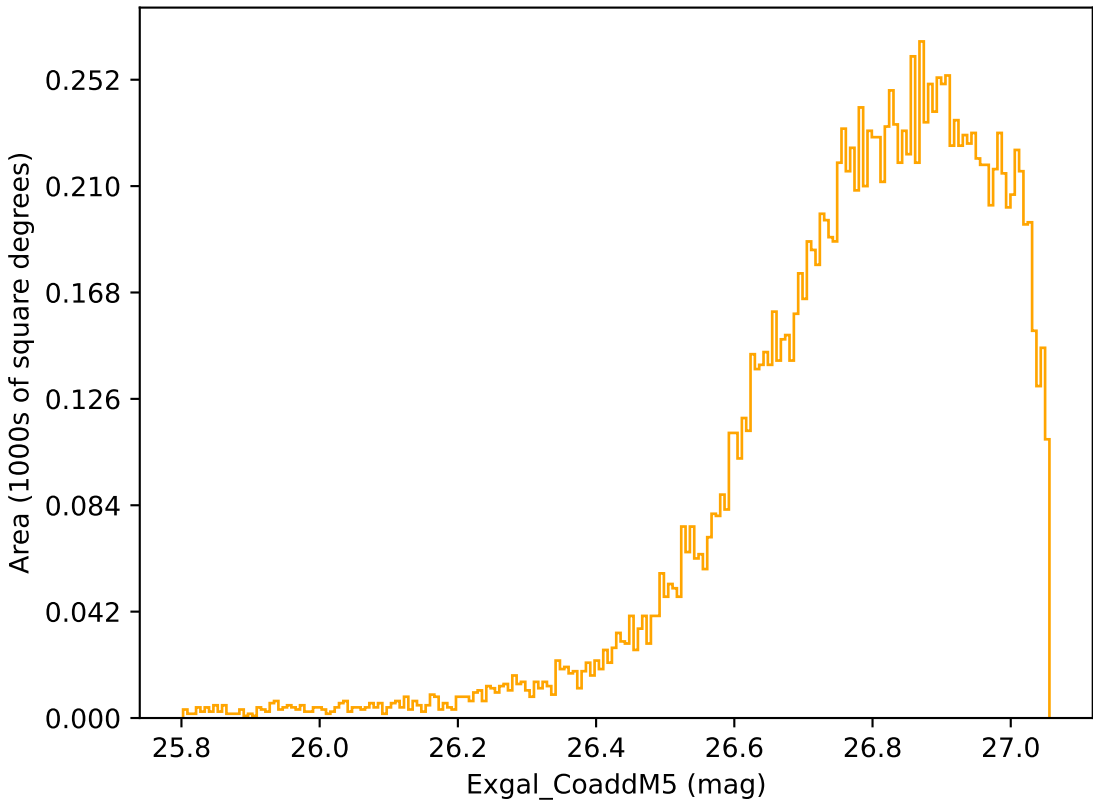
too_elab_r64_d3_giz_v3.4_10yrs WFD r band: Exgal_CoaddM5
