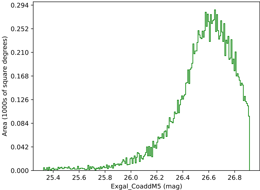
too_elab_r64_d3_giz_v3.4_10yrs WFD g band: Exgal_CoaddM5
