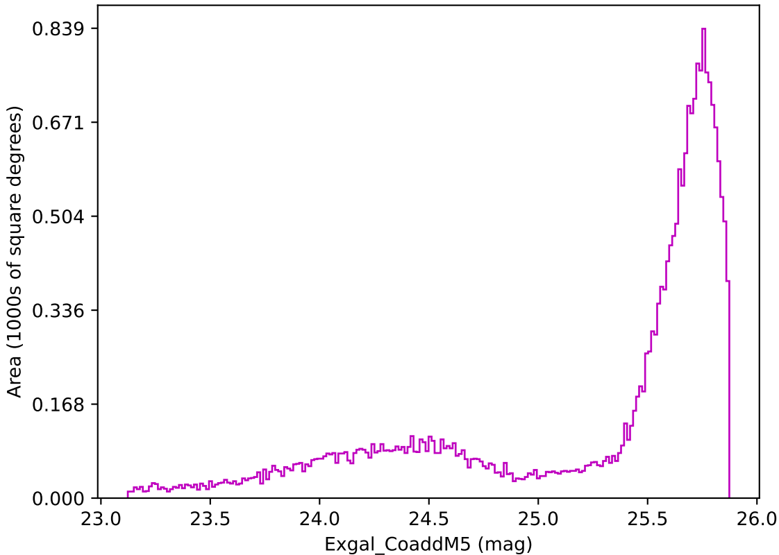
too_elab_r64_d3_giz_v3.4_10yrs All sky z band: Exgal_CoaddM5
