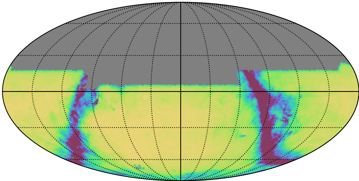
too_elab_r64_d3_giz_v3.4_10yrs All sky u band: Exgal_CoaddM5
